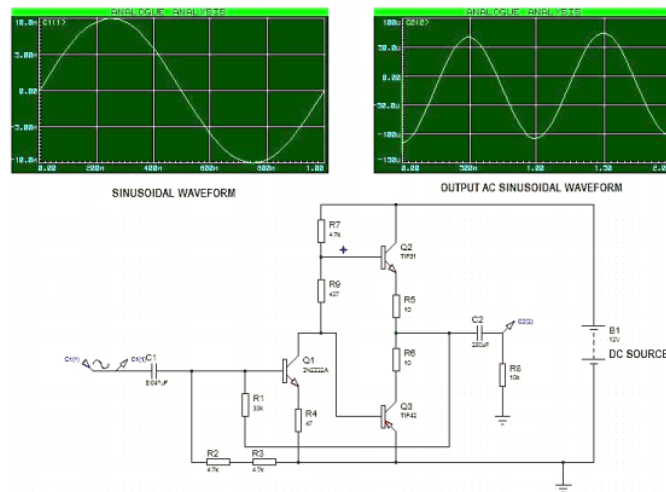
Figure 6. Simulation of Push-Pull Amplifier
