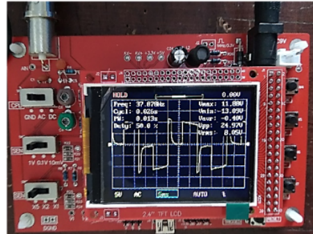
Figure 5. Experimental of Assembled 3-phase Inverter
