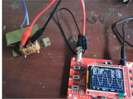
Figure 2. Experimental Sine Waveform of Transformer CT
