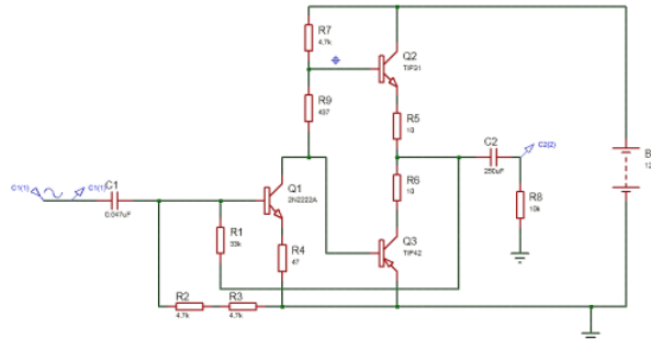
Figure 1. Proposed Push-Pull Amplifier.
