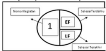
Gambar 4. Node CPM
