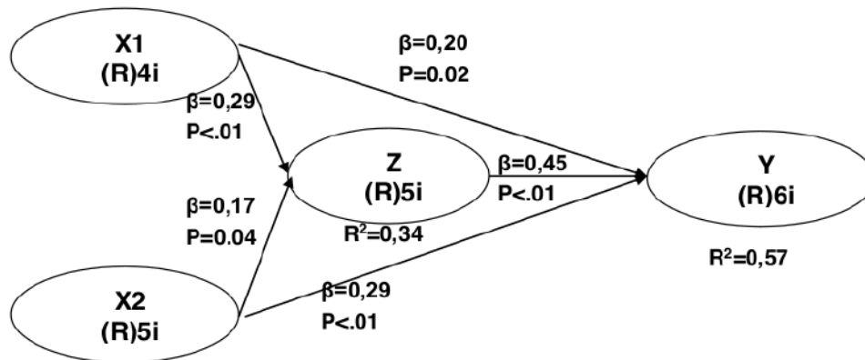
Figure 1: Path Analysis
