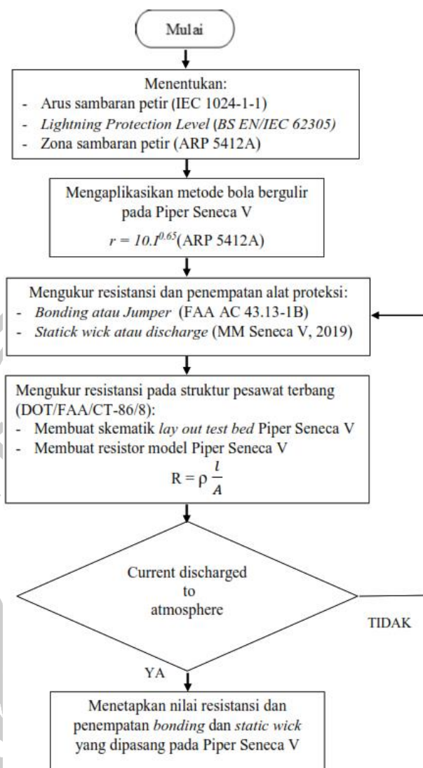
Gambar 3. Diagram Urutan Penelitian
