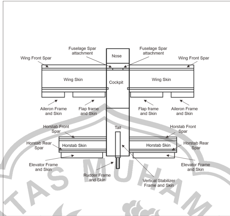
Gambar 8 Test Bed Model Piper Seneca V (DOT/FAA/CT-86/8, 1987)
