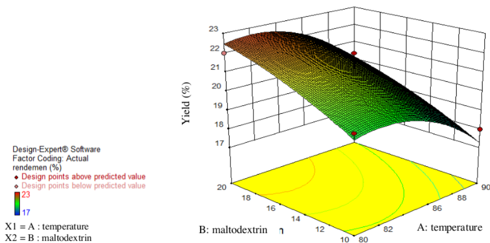
Figure 4. Yield response of noni powder based on temperature and maltodextrin concentration
