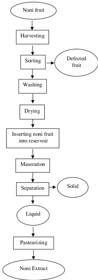
Figure 1. Flow Chart of Noni Liquid Making
