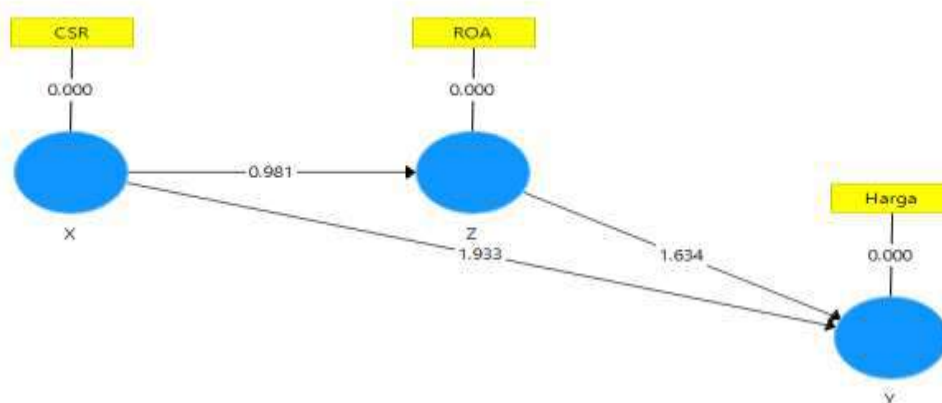
Figure 1 PLS Model
