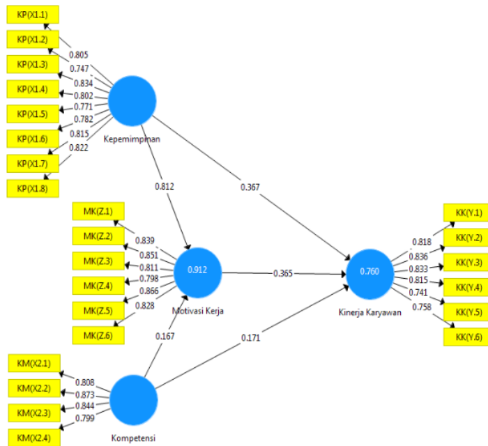
Figure 2. Model Pengujian Partial Least Square Warp PLS 3.0
