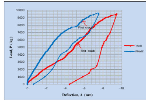
Fig. 5. The relationship of load ( P ) vs deflection ( \Delta ) of bridge frame
