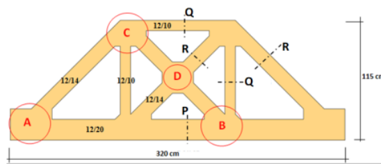
Fig. 2. The dimensions of the bamboo reinforced concrete bridge frame
