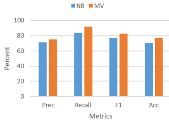
Figure 3. Performance of NB vs. MV.
