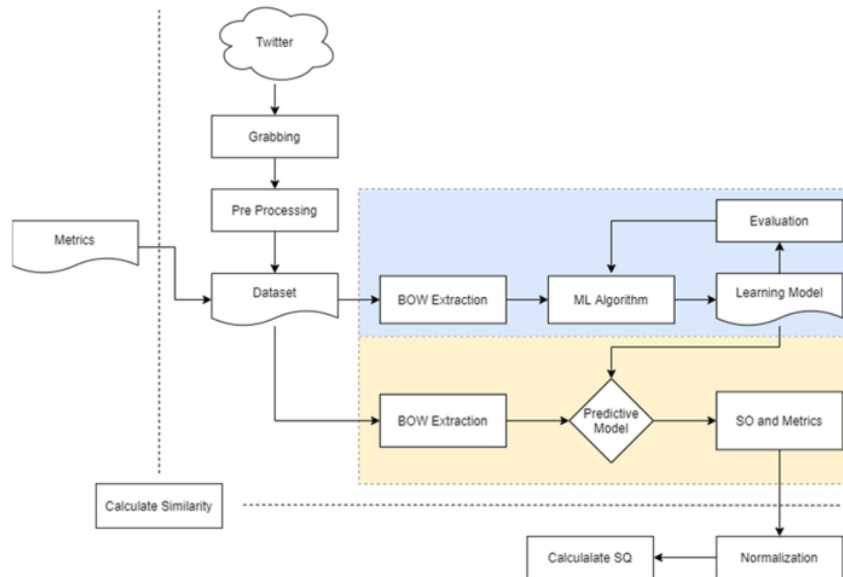
Figure 1. The framework of the service quality calculation.
