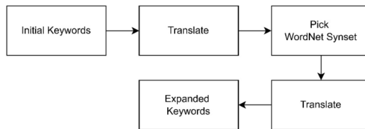
Figure 6. Initial keywords extension.
