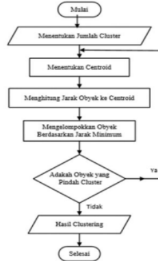
Gambar 3. Flowchart Alur Algoritma K-Means
