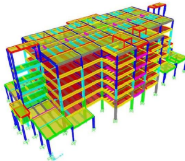
Figure 3. 3D Structural modeling soil site class
