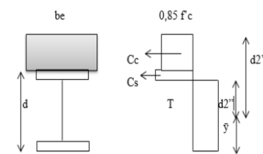
Gambar 3.3 Sumbu netral plastis & distribusi tegangan
