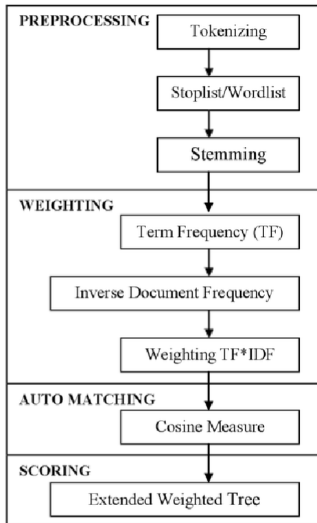
Gambar 1. Metode Penelitian Preprocessing, Weighting, Auto Matching, Scoring
