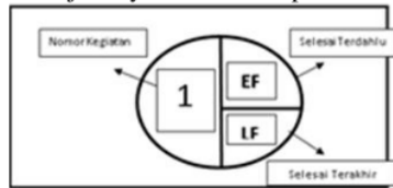
Gambar 4. Node CPM
