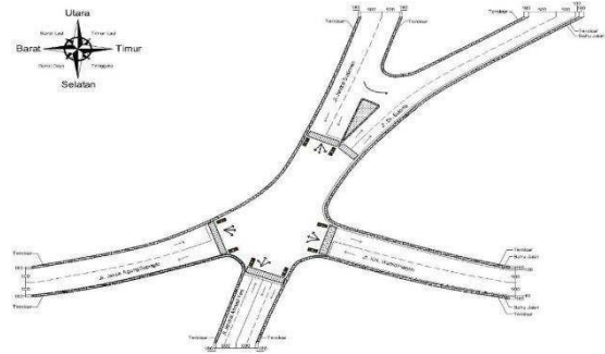
Gambar 3. Geometrik Simpang Lima
