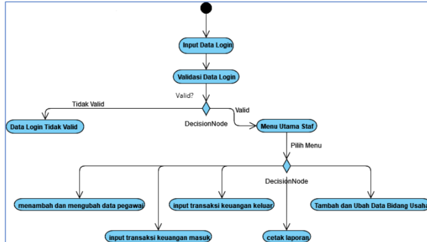
Gambar 4 Activity Diagram
