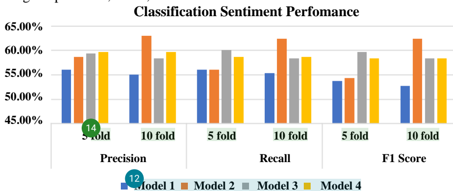
Figure 4: Comparison of Classification Performance
