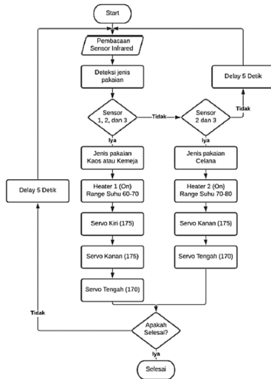
Gambar 5. Flowchart Sistem Alat
