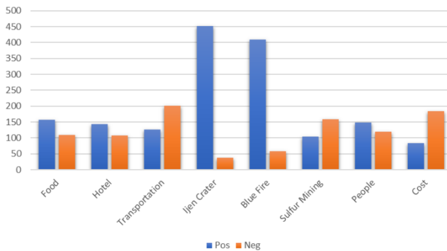
Fig 5. The result of aspect based sentiment analysis
