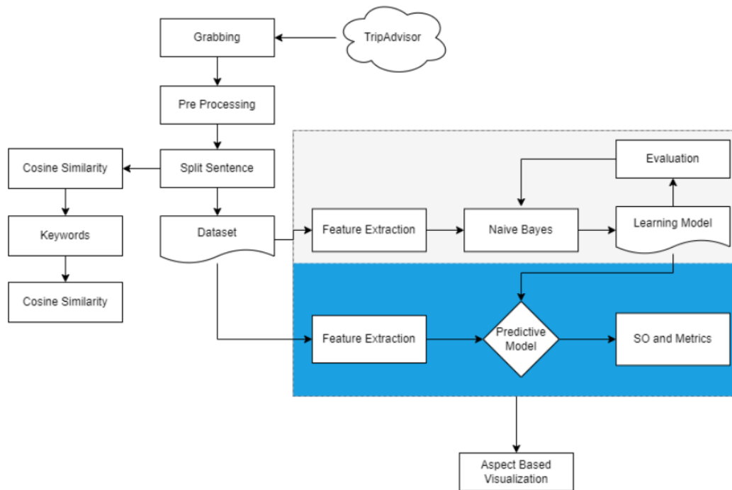
Fig 1. Framework of the proposed method
