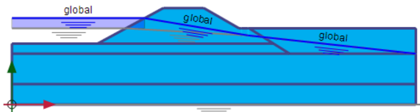
Figure 14: geometry of dam water level during Rapid Drawdown
