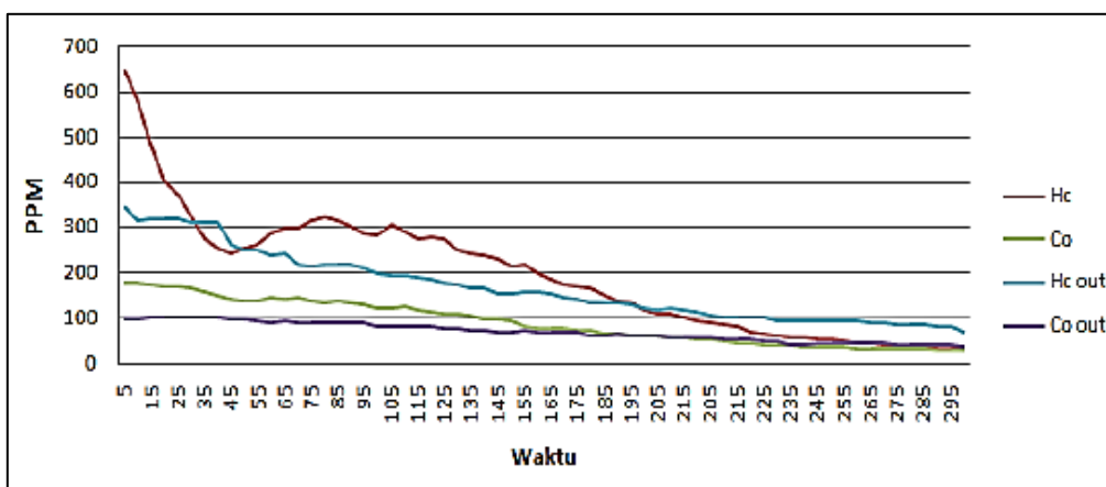
Gambar 13. Percobaan 64 RPM
