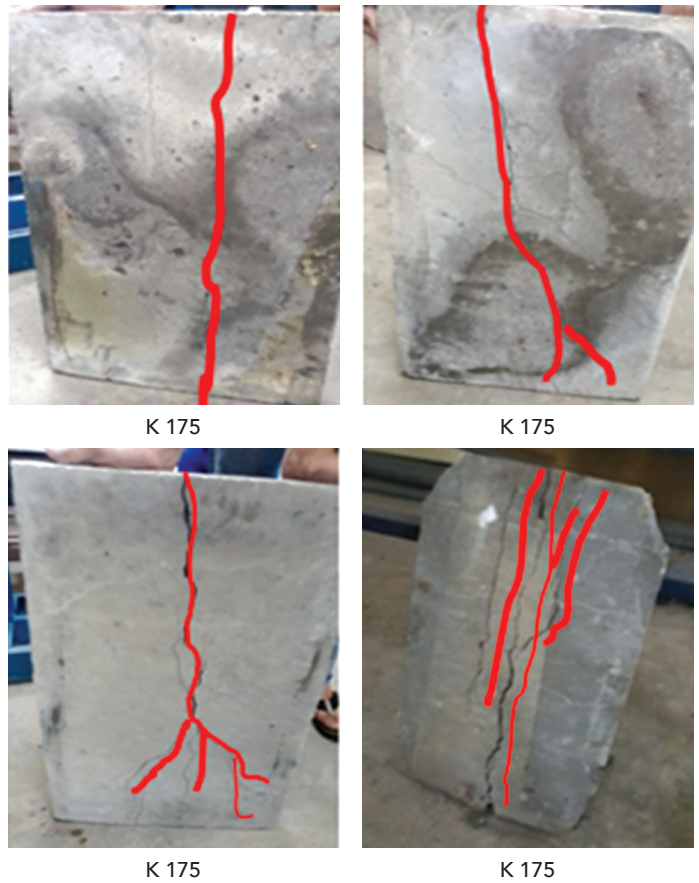
Figure 6: The cracking behavior of concrete slabs with a thickness of 3.5 cm
