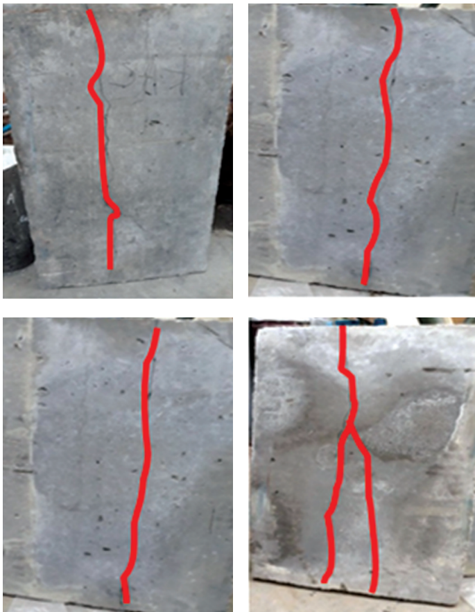
Figure 5: The cracking behavior of the concrete gate with a thickness of 3 cm
