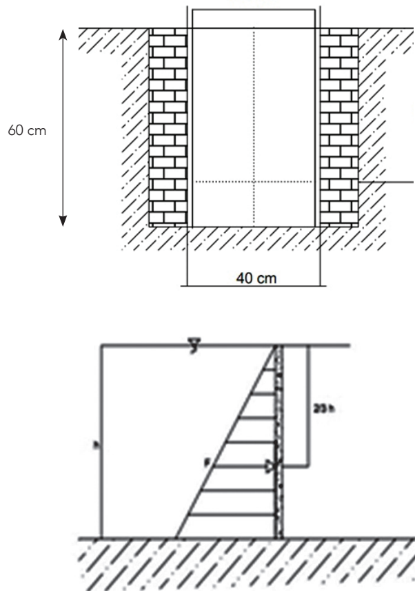
Figure 2: Distribution of forces acting on a concrete gate
