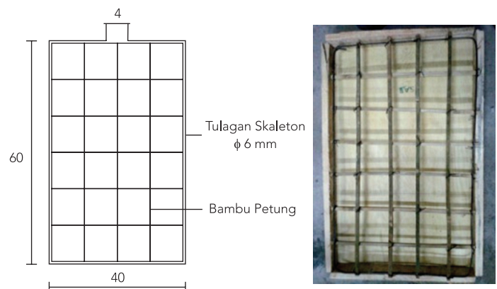
Figure 1: Selection of bamboo petung and how to mount reinforcement
