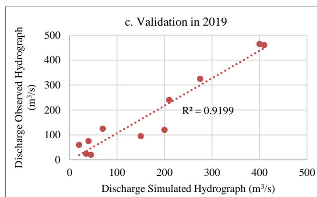
Figure 11. The results of the regression distribution plotting (a) Calibration of the Lempake Dam in 2017; (b) Calibration of the Lempake Dam in 2018; and (c) Validation of Lempake Dam in 2019
