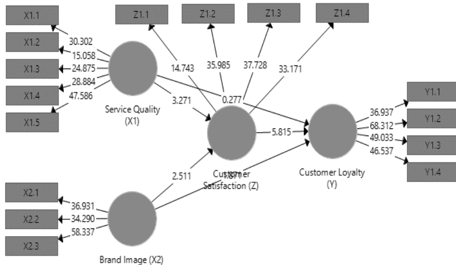
Gambar 1. Bootstrapping Model
