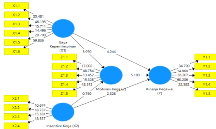
Gambar 2. Hasil Analisis Inner Model
