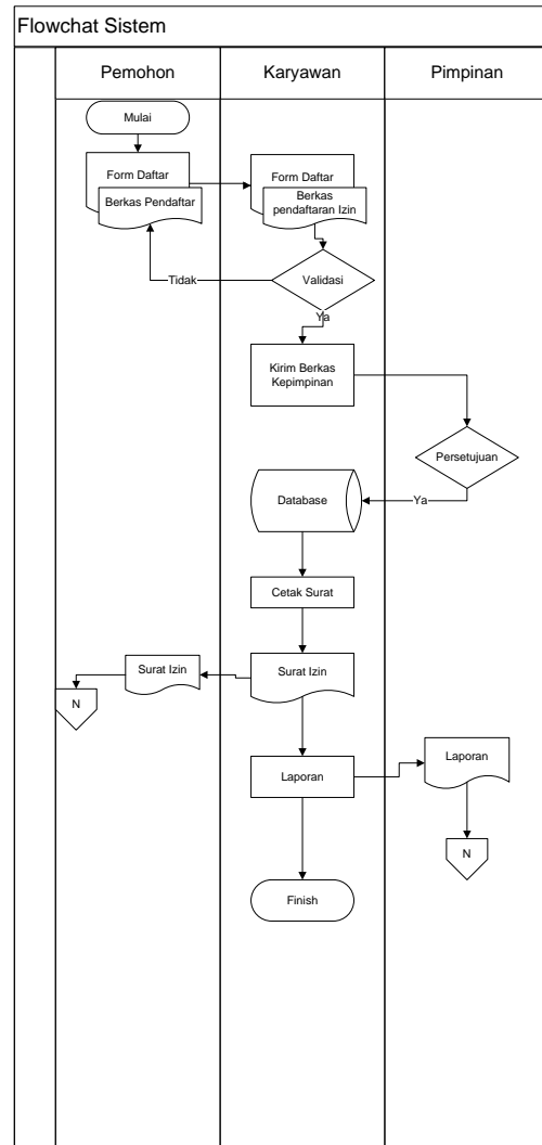
3.1 Flowchat Sistem
