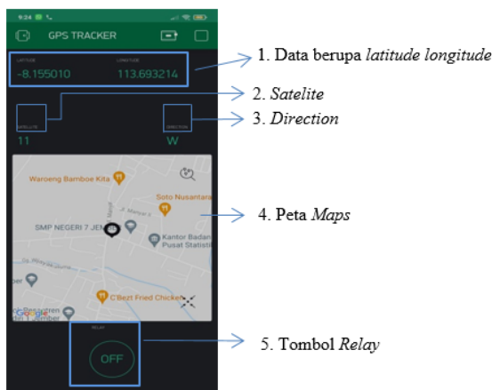
Gambar 9. Desain software
