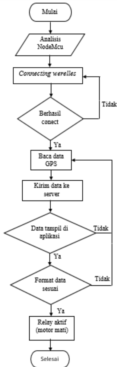
Gambar 7. Flowchart sistem alat
