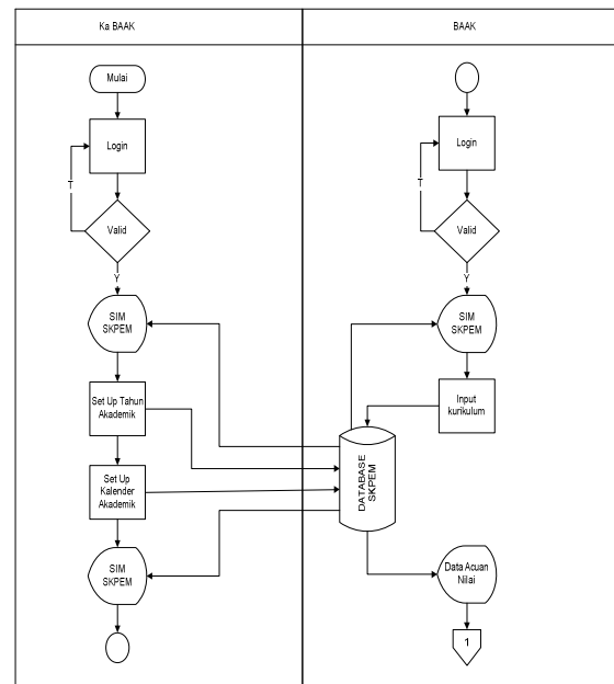
Gambar 3.1 Flowchart Kurikulum
