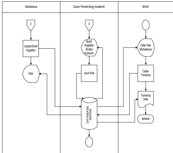
Gambar 3.3 Flowchart Penilaian
