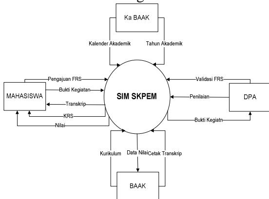
Gambar 3.4 Data Flow Diagram
