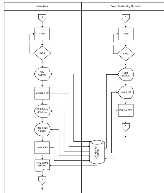
Gambar 3.2 Flowchart KRS
