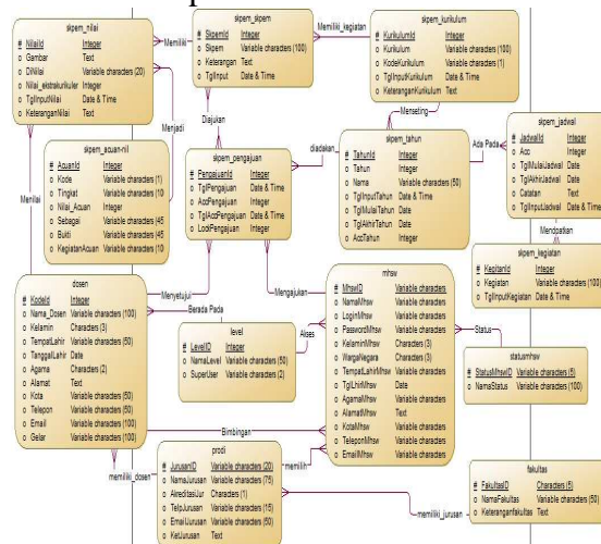
Gambar 3.5 Conceptual Data Model
