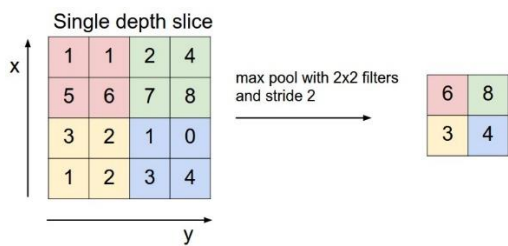
Gambar 2. Contoh Operasi Max Pooling
