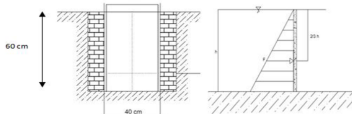
Fig 2. Distribution of forces acting on a concrete gate
