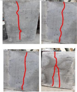
Fig 5. The cracking behavior of the concrete gate with a thickness of 3 cm
