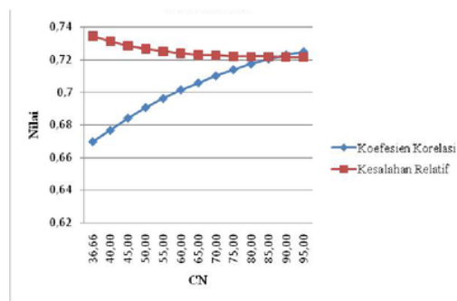
Figure 13. Graph of Correlation Value Calculation And Relative Error to CN Value
