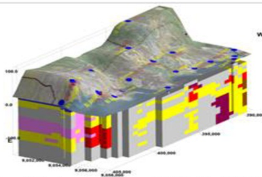
Figure 2. The interpretation of rock 3D Model with IP2Win
