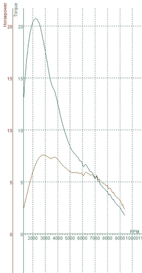
DATA FOR TEST: SCOOPY FI STD PERTAMAX TEST 3
