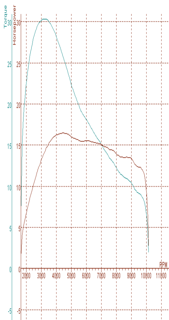
DATA FOR TEST: SCOPY FT PERTAMAX 1
