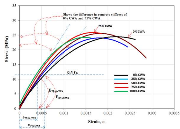
Fig. 10. The stress-strain relationship of the ceramic concrete (CWA)
