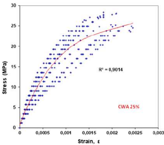
Fig. 4. The stress-strain relationship of the ceramic concrete (25% CWA)
