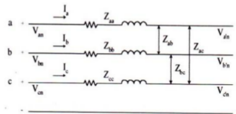
Figure 1 Channel Model Three Phase
