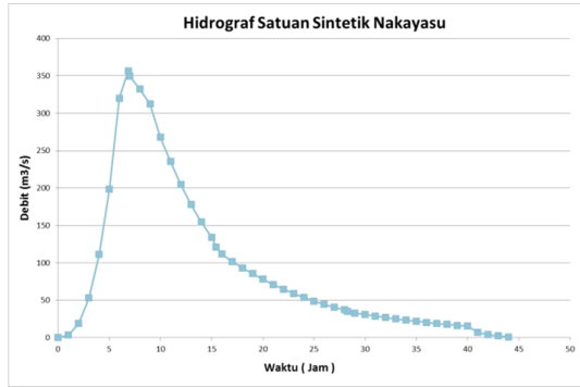
Gambar 3. Hidrograf HSS Nakayasu
