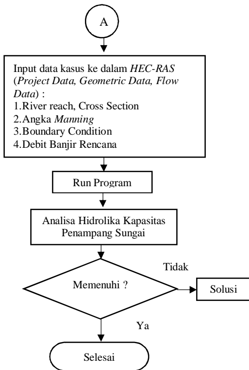
Gambar 2. Flow Chart
