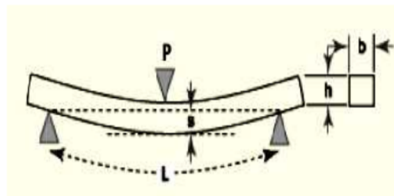
Gambar 3. Penampang bending (balok) Sumber : ASTM D 790, 1997
