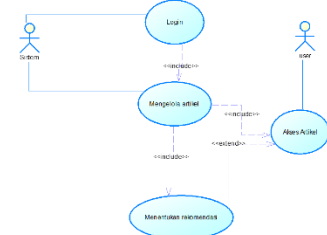
Gambar 3.3 usecase diagram
