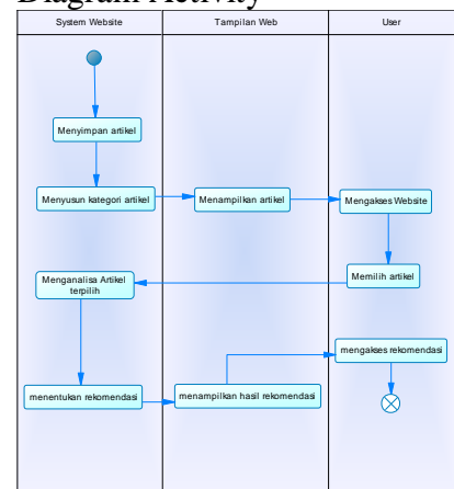
Gambar 3.4 Diagram Activity
