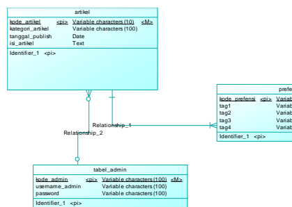
Gambar 3.5 Desain Database
