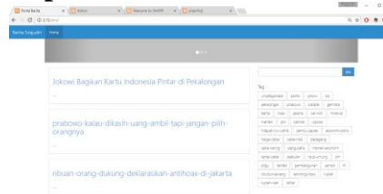
Gambar 4.1 Tampilan Website
