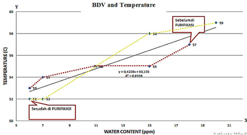
Figure 5. Value of water content vs temperature
