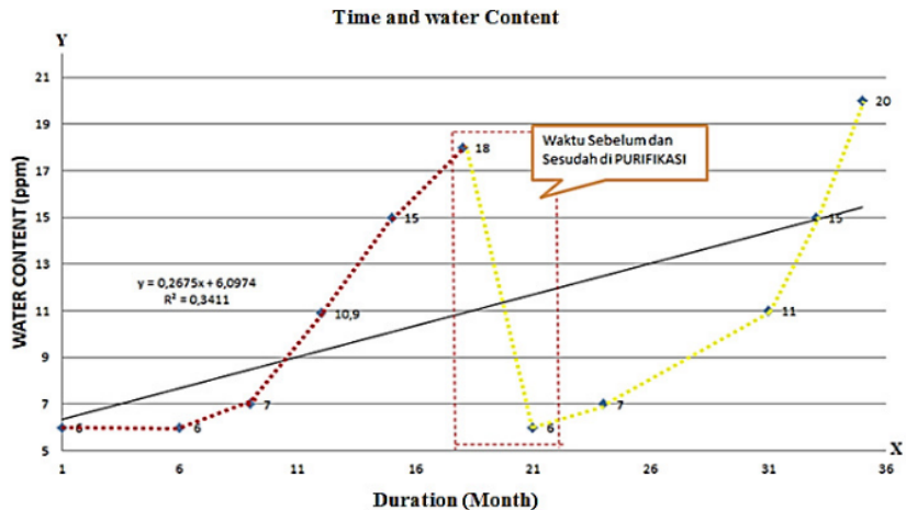
Figure 6. Water content vs time curve value
