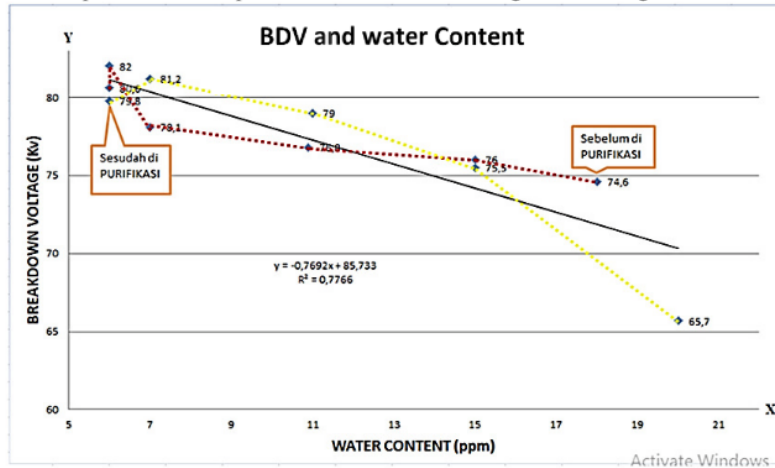
Figure 4 Water Content Vs BDV Value Curve
