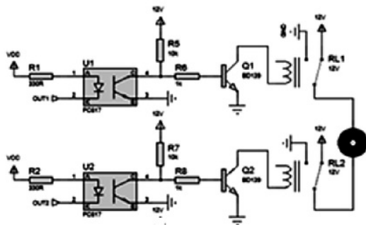
Gambar 5. Diagram Perancangan Sistem Hardware
