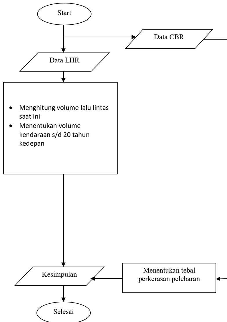
Gambar 3.1 Diagram Penelitian
