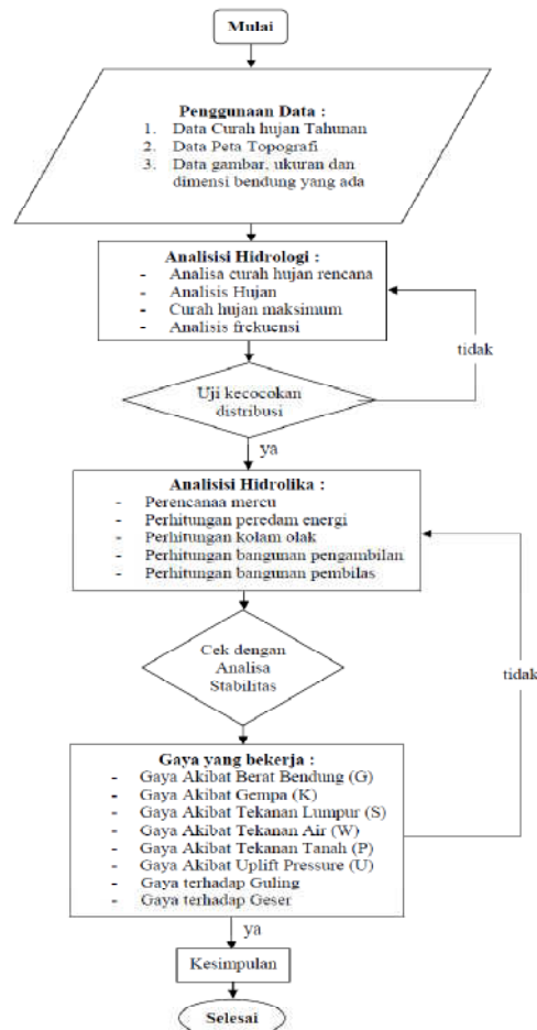
Gambar. Flow Chart Diagram
