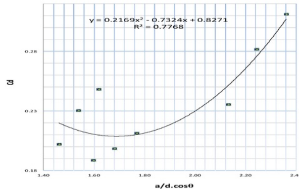
Figure 13 Relationship between coefficients discharge (Cd) with a/d Cos θ in Sub-critical flow (Fr < 1)
