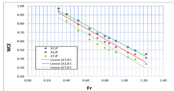
Figure 9 Relationship of Froude numbers ( Fr ) and water catchment (WCE) on A_{ro1}
