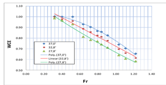
Figure 11 Relationship of the Froude number (Fr) and water catchment (WCE) on Aro3
