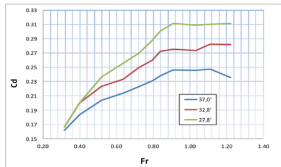
Figure 6 Relationship of Froude number (Fr) and the discharge coefficient (Cd) on Aro 1
