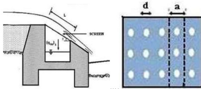
Figure 2 schematic flows on tyrol weir with a perforated hollow screen
