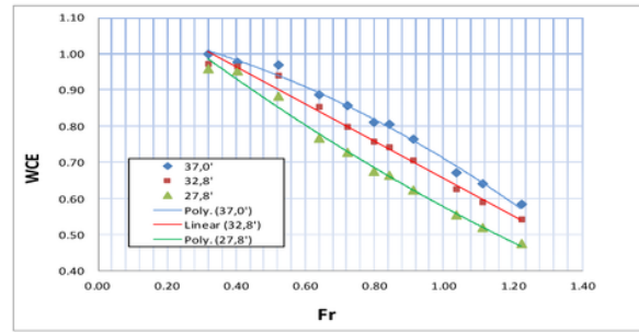
Figure 10 Relationship of Froude numbers (Fr) and water catchment (WCE) on Aro2
