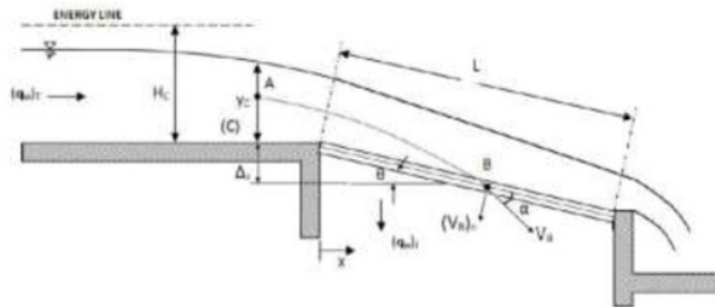
Figure 5 Schematic of water flow entering the tyrol weir
