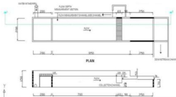
Figure 3 Layout of physical model test of tyrol weir in laboratory with a circular perforated plate screen
