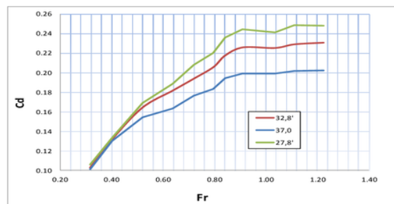
Figure 7 Relationship of the numbers Froude (Fr) and the discharge coefficient (Cd) on Aro 2
