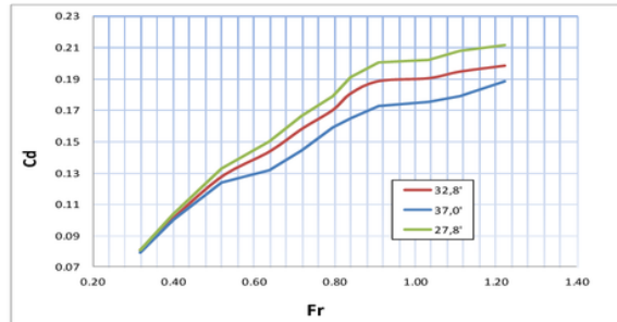
Figure 8 Relationship of Froude numbers ( Fr ) and the discharge coefficient ( C_d ) on A_{ro3}
