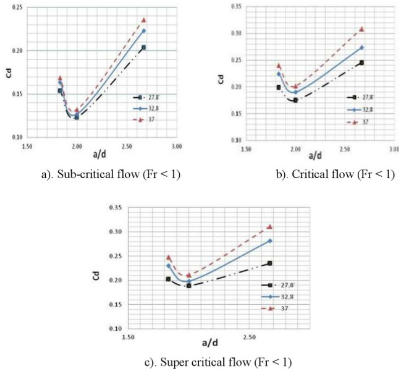
Figure 12 The value of coefficient of discharge (Cd) and distance ratio between holes (a/d)
