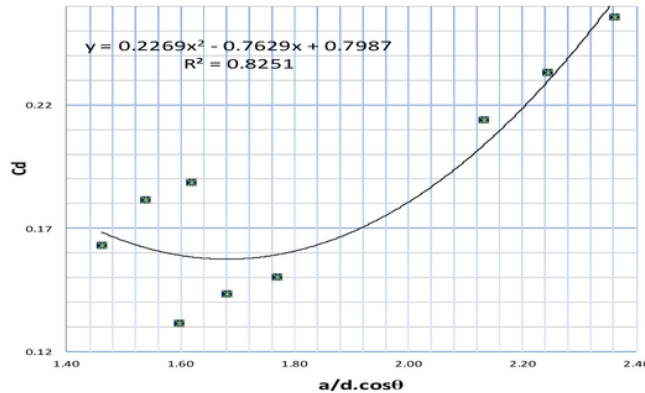
Figure 14 Relationship between coefficients discharge ( C_d ) with a/d \cos \theta in Super critical flow ( Fr > 1 )
