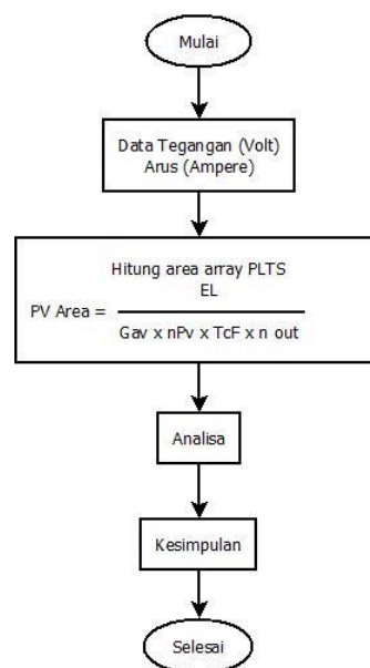
Gambar 3. Flowchart Analisa
