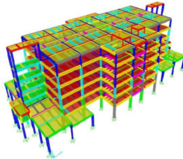
Figure 3. 3D Structural modeling soil site class
