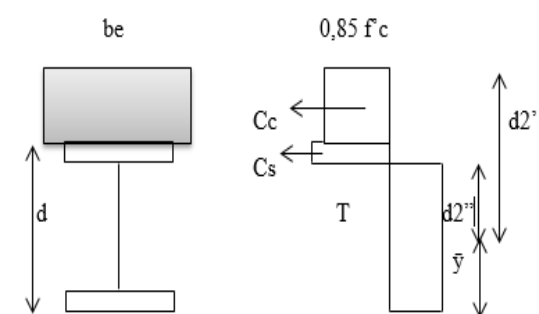
Gambar 3.3 Sumbu netral plastis & distribusi tegangan
