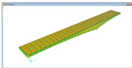
Gambar 9. Gambar SAP2000 Tampak 3-d Extrude View
