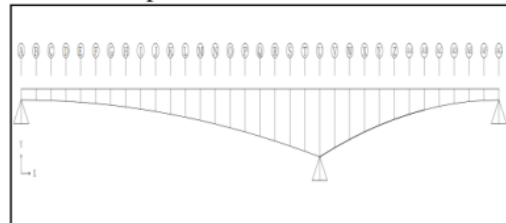
Gambar 6. Gambar SAP2000 Tampak X-Z
