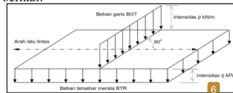
Gambar 4. Beban Lajur "D" (Sumber : RSNIT-02-2005)
