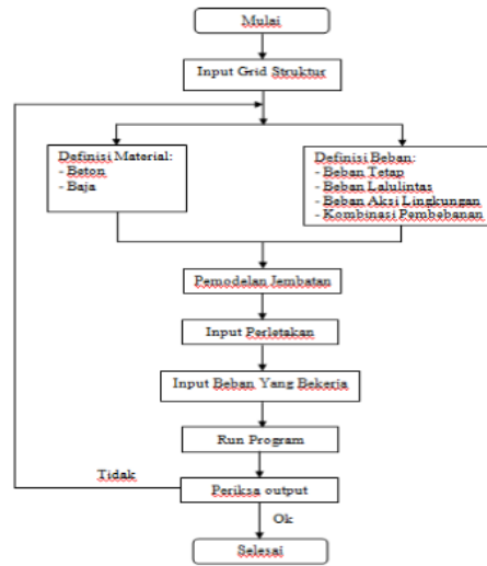
Gambar 3.2 Diagram Alir Program SAP2000
